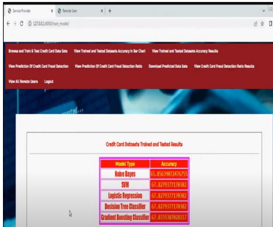
Fig.7. Algorithms applied.
