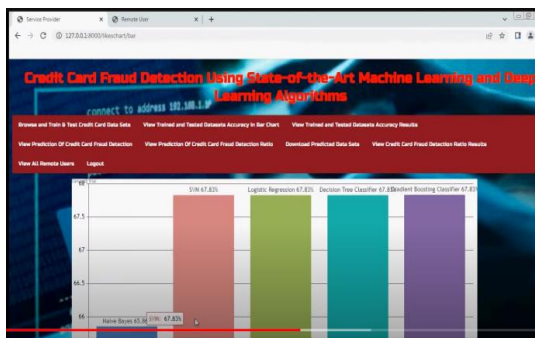
Fig.8. Prediction Graphs.
