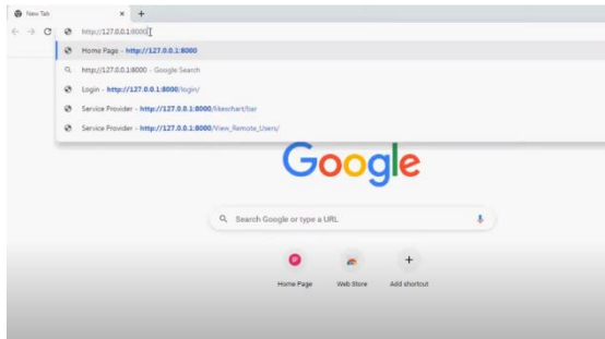
Fig.1. Home page.
