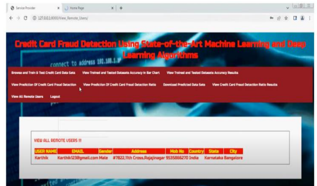
Fig.4. User details.
